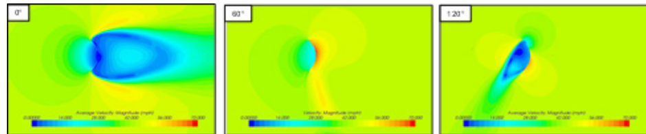
▲ Flow velocity contours at dish midplane
