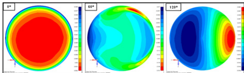
▲ Delta pressure contours across dish
